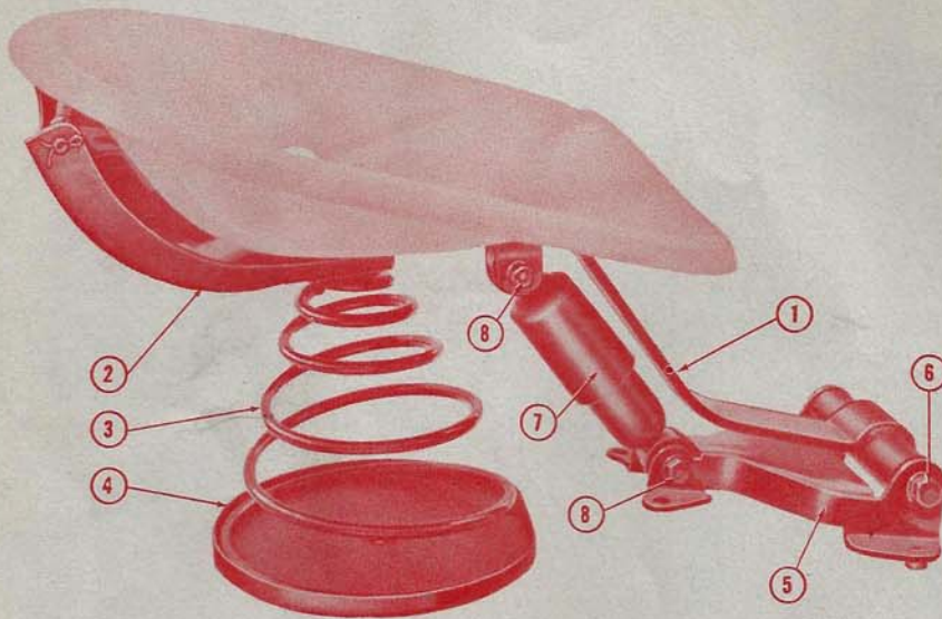
Part No. 230200 - Tractor Seat - Less Seat Pan
