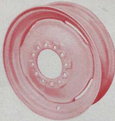
8N 1015-B2 Heavy Duty Front Wheel (Use w/6.00" - 16" Tires)
