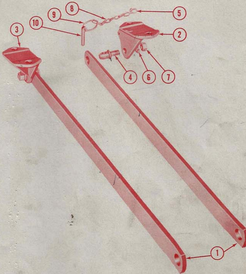
Model 22-41 Stabilizer Link Kit Assembly
