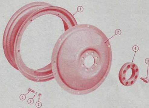
Dual Rear Wheel Assembly
